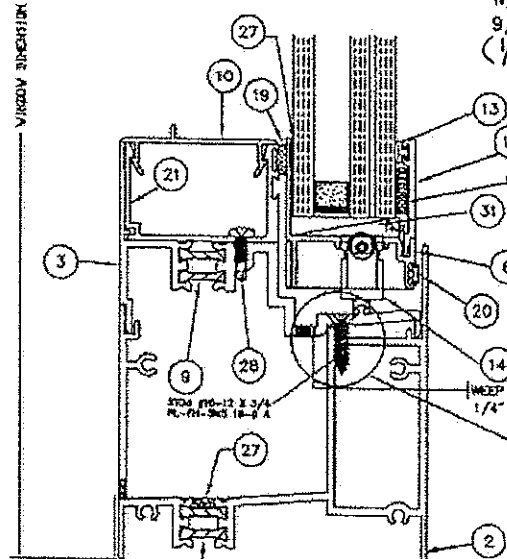
2 SILL
